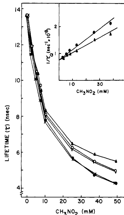
FIGURE 2: Nitromethane quenching patterns of PySA-labeled, AcChR-enriched membranes in the presence of cholinergic ligands: (V) control (no ligands are added); (O) 10^{-6} M carbamylcholine; (Δ) 10^{-3} M carbamylcholine; (●) \alpha -bungarotoxin (2-fold molar excess to \alpha -bungarotoxin binding sites); (X) \alpha -bungarotoxin followed by 10^{-3} M carbamylcholine. Conditions for the preparation of the samples are indicated under Materials and Methods and in Table II. Insert: Stern-Volmer plots of nitromethane quenching on PySA-labeled AcChR-enriched membranes in the presence of 10^{-3} M carbamylcholine (Δ) and \alpha -bungarotoxin (●).
